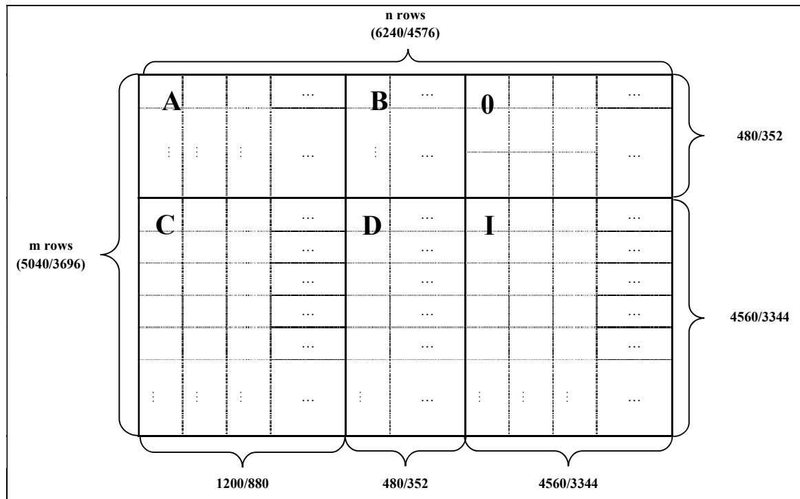
Figure 10: LDPC Submatrices
